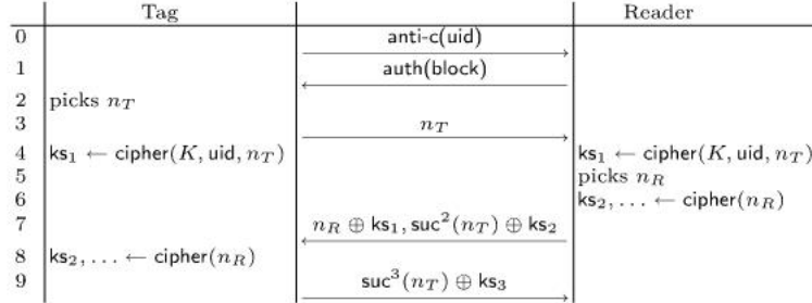
Fig. 3. Authentication Protocol
