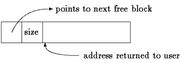
A block returned by malloc
