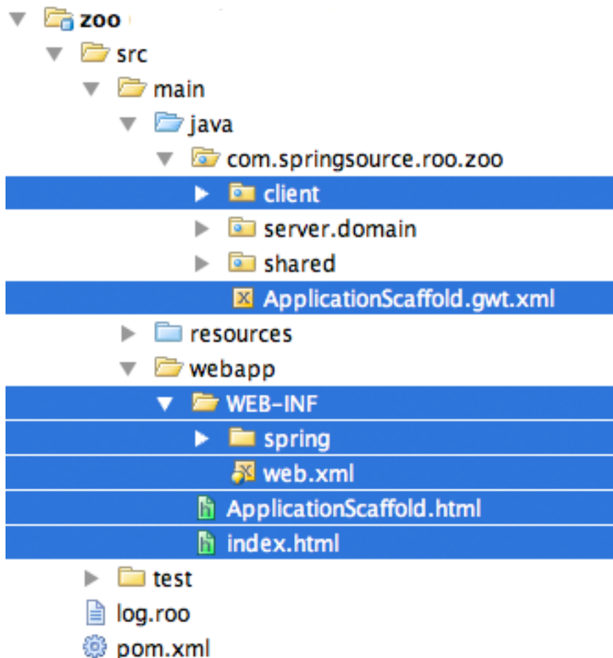
Figure 12.2. Figure GWT.2: New packages and files created from running “gwt setup”
